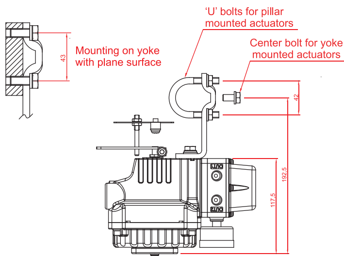
Mounting to linear actuators to IEC 60534 6-1
